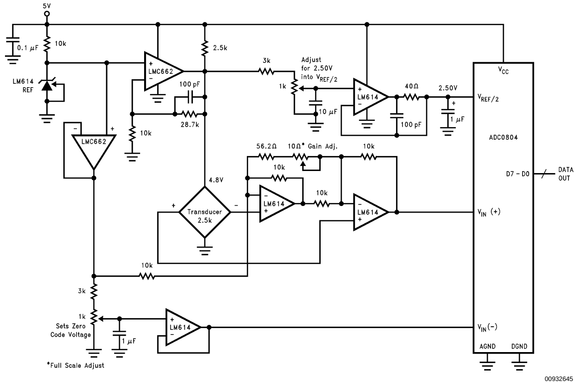
FIGURE 15. Transducer Data Acquisition System. Set zero code voltage, then adjust 10\Omega gain adjust pot for full scale.
