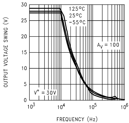
Output Swing, Large Signal
